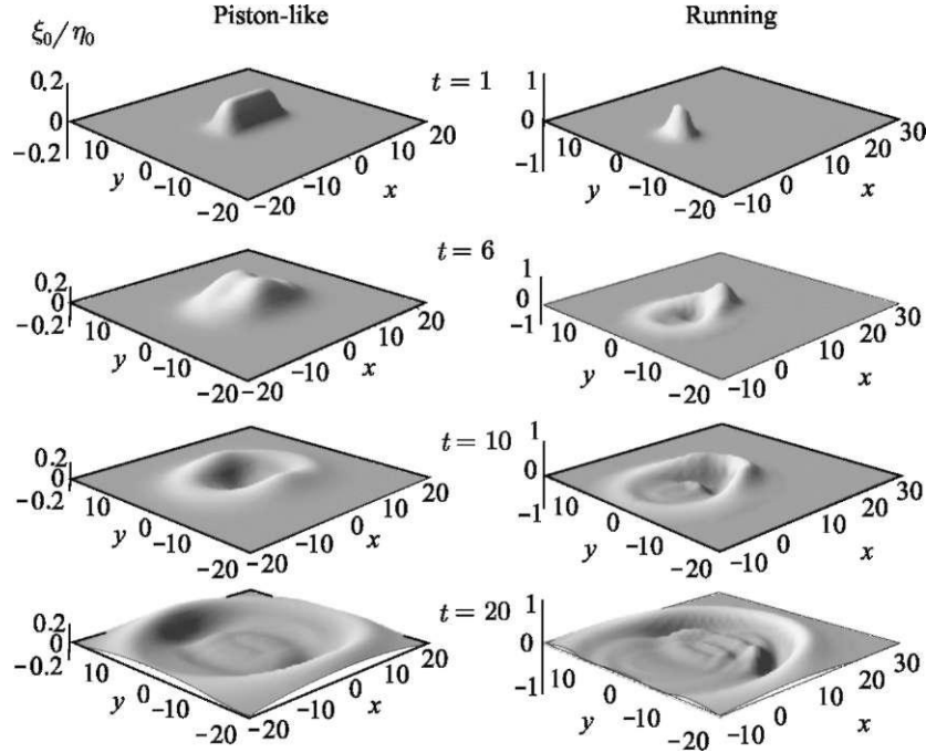
Fig. 2.29 Free-surface perturbations, caused by piston-like and running displacements of the bottom with parameters a = 6 , b = 2 , v = 2 ( \tau = 6 ). Calculations are performed for the time moments t indicated in the figure
