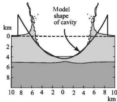
Fig. 4.16 Shape of cavity formed in water by a falling meteorite: comparison of results of numerical simulation [Crawford, Mader (1998)] and of idealized model (formula (4.36) with account of relations (4.41) and (4.43)). Calculations are performed for a time moment of 25 s, an asteroid diameter of 500 m, a fall velocity of 20 km/s, a density of 3.32 g/cm 3 and ocean depth of 5 km (Adapted from [Ward, Asphaug (2000)])
