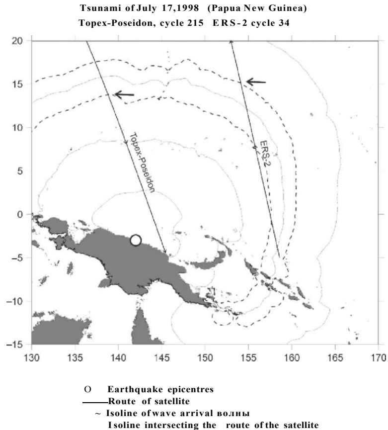
Fig. 6.12 Map of Pacific Ocean region adjacent to the island Papua New Guinea with isoUnes of arrival times of the 1998 tsunami (in 1 h steps). Shown are the routes of the satelUtes Topex-Poseidon (circuit 215-18) and ERS-2 (circuit 34-304), which intersect the tsunami wave front. The crossing points of the routes and the respective isolines of the tsunami front arrival times (dashed line) are indicated by arrows (The figure is taken from [Zaichenko et al. (2004)])
