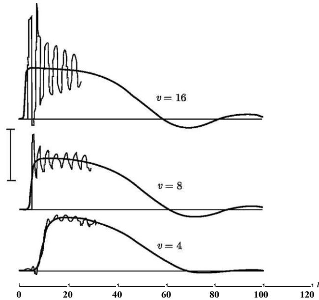
Fig. 3.6 Time evolutions of surface displacements of liquids at the centre of the active zone for different displacement propagation velocities v . The thick and thin lines correspond to incompressible and compressible liquids, respectively
