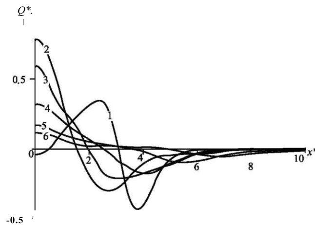
Fig. 3.26 Characteristic form of function Q^*(x^*, t^*) . Curves 1-6 correspond to t^* = 4, 8, 12, 16, 20, 24 . The source parameters: m = 8 s, L = 40 km, H = 4 km
