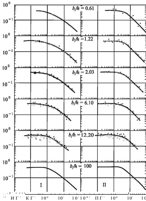
Fig. 2.19 Amplitude of wave, excited by piston-like basin bottom displacement of amplitude b_0 as function of the displacement duration \tau . Adapted from [Hammack (1973)]
