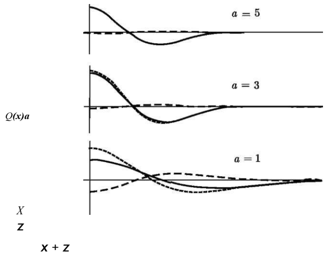
Fig. 3.20 Characteristic form of function Q(x) and of its components X(x) and Z(x) . The calculation is performed for the space distribution of the ocean bottom oscillation amplitude u_1 for a = 1, 3 and 5
