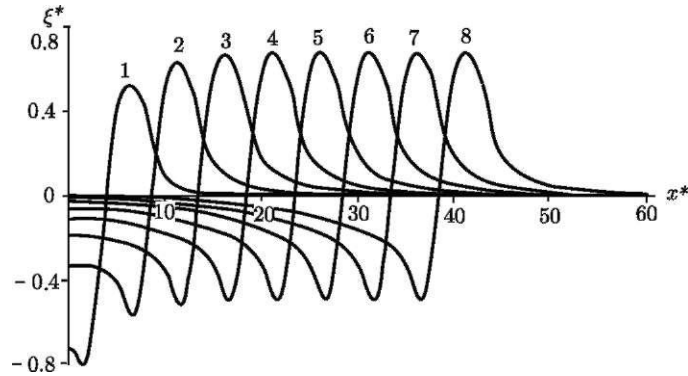
Fig. 3.27 Profiles of gravitational waves formed by a 'non-linear source'. Curves 1-8 are calculated for consecutive moments of time separated by intervals of 100 s. The source parameters: m = 8\text{ s} , L = 40\text{ km} , H = 4\text{ km}
