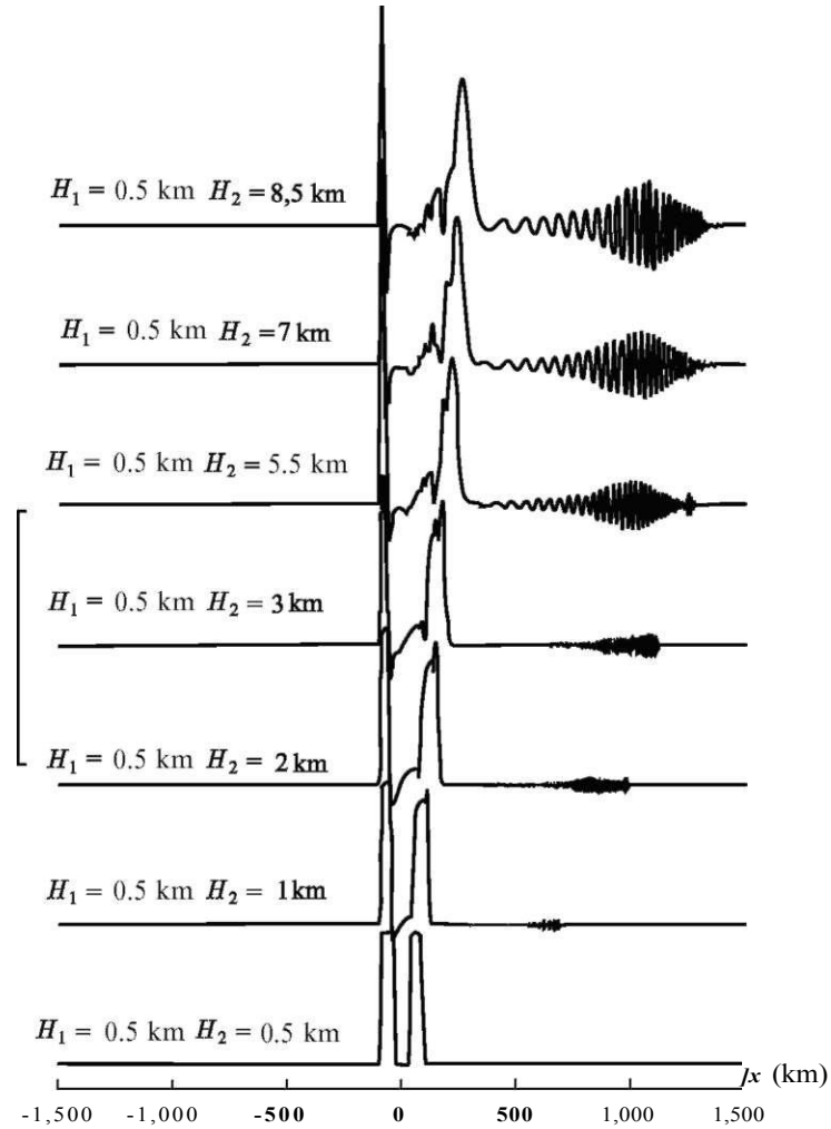
Fig. 3.9 Perturbation of free surface at time moment t = 1,000 s
