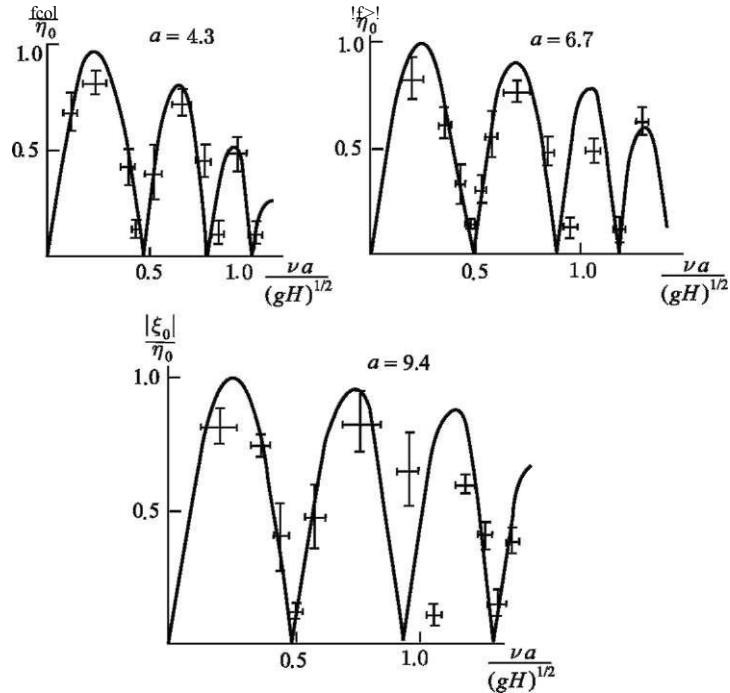
Fig. 2.28 Comparison of experimental and theoretical dependences of amplitudes of excited progressive wave versus frequency of bottom oscillations
