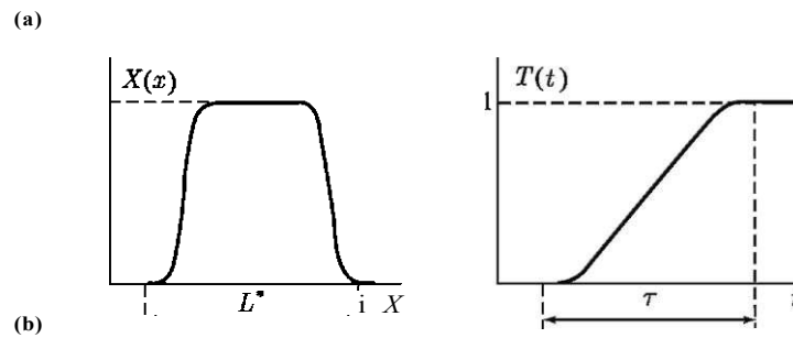
Fig. 3.8 Shape of calculation region (a). Space-time law of motion of bottom (b)
