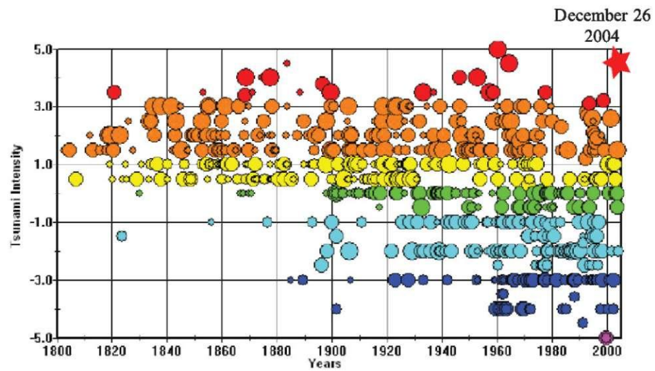
Plate 2 Tsunamis of the Pacific region in the 'intensity-time' plane (see also Fig. 1.6 on page 19)
