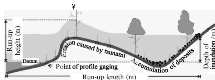
Fig. 6.9 Scheme for gaging the main characteristics of tsunami manifestations along the topographic profile
