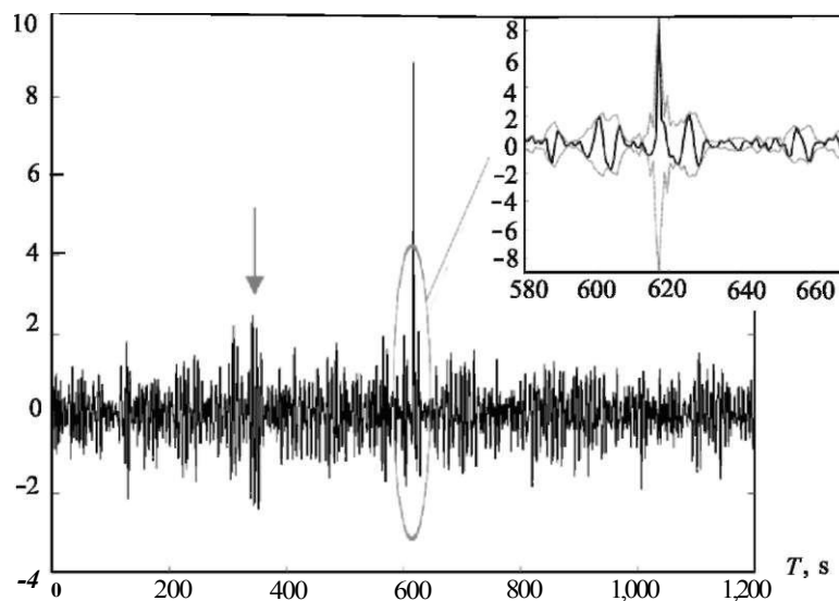
Fig. 1.8 Anomalous wave, registered in the Black Sea on November 22, 2001
