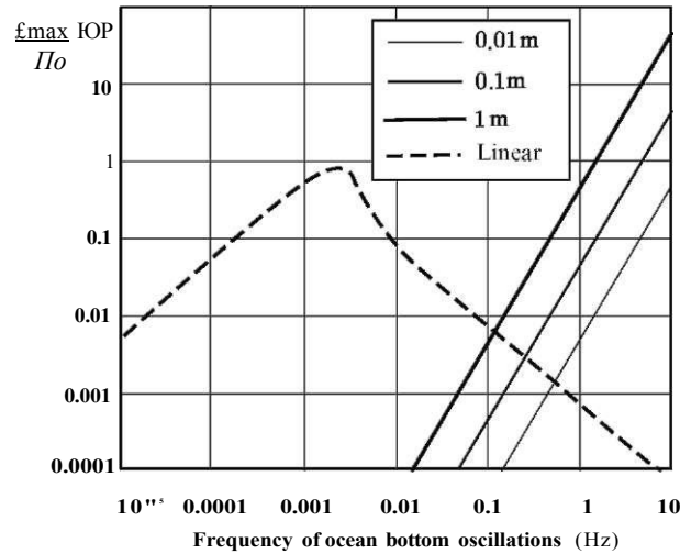
Fig. 3.23 Amplitude of gravitational waves, excited by oscillations of ocean bottom, versus oscillation frequency: linear and non-linear responses. Calculations are performed for exponential distribution of amplitude of bottom oscillations for a = 10 km and ocean depth of 1 km
