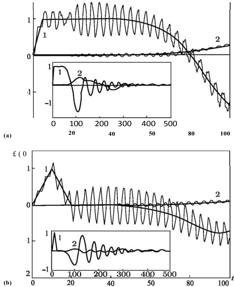
Fig. 3.2 Examples of time evolutions of free-surface perturbations of compressible (thin line) and incompressible (thick line) liquids, caused by displacements of the bottom of duration m = 5 with a residual deformation (a) and of duration m = 20 without any residual displacement (b). Curves 1, 2 correspond to r = 0, 20 , respectively. Calculation were performed for R = 10
