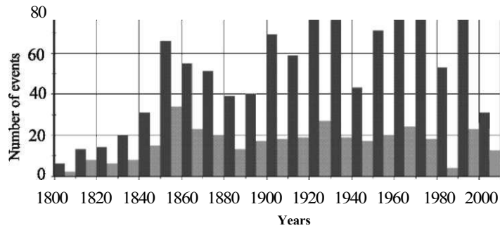
Fig. 1.5 Recurrence of tsunamis (number of events per decade) in the Pacific region between 1800 and 2005. The dark colour shows all the known tsunamis, the grey colour indicates tsunamis of intensity I^1 according to the Soloviev-Imamura scale
