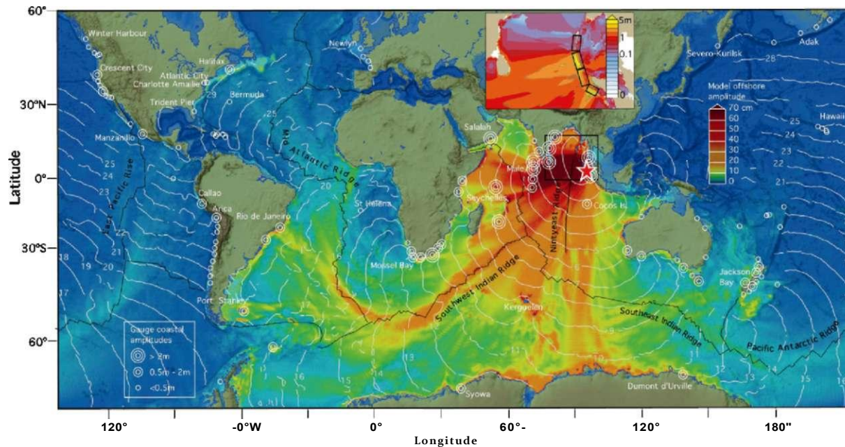
Plate 6 Global chart showing energy propagation of the 2004 Sumatra tsunami calculated from MOST. Filled colors show maximum computed tsunami heights Q during 44 hours of wave propagation simulation. Contours show computed arrival time of tsunami waves o . Circles denote the locations and amplitudes of tsunami waves in three range categories for selected tide-gauge stations g . Inset shows fault geometry of the model source and close-up of the computed wave heights in the Bay of Bengal J . Distribution of the slip among four subfaults (from south to north: 21 m, 13 m, 17 m, 2 m) provides best fit for satellite altimetry data and correlates well with seismic and geodetic data inversions (Reprinted from [Titov et al. (2005)] by permission of the publisher (see also Fig. 5.10 on page 221)
