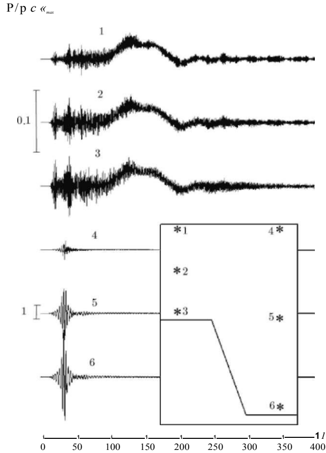
Fig. 3.11 Dynamic pressure, calculated as function of time at fixed points. The pressure is normalized to the quantity p c v_{max} , where v_{max} is the maximum velocity of movement of the ocean bottom. The scale units for realizing 1-3 and 4-6 are different (indicated in the figure for curves 2 and 5, respectively)
