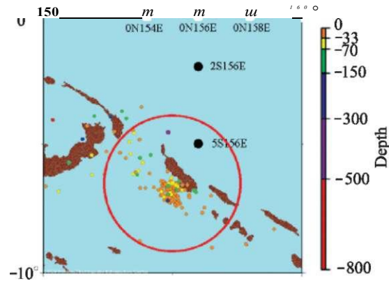
Plate 16 Earthquake epicenters in the vicinity of Bougainville Island for the period of 20.04.1996-31.05.1996. The center of the red circle of radius 300 km is at the point 6.528 S, 155.00 E (epicenter of earthquake of maximum amplitude). The black circles indicate the location of TAO Array stations (see also Fig. 7.1 on page 279)
