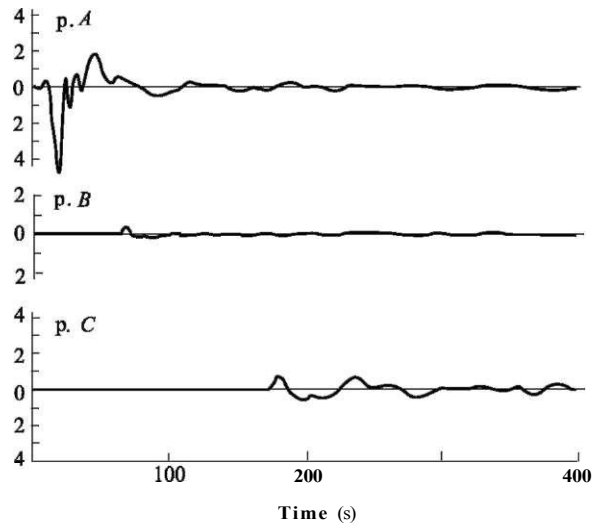
Fig. 4.4 Results of calculations of level oscillations at points A, B and C, the locations of which are indicated in Fig. 4.2. Adapted from [Rabinovich et al. (2003)]
