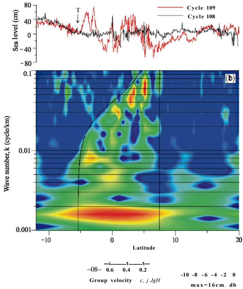
Plate 15 (a) Altimetry sea-level taken along track 129 of the Jason-1 satellite for Cycle 109 and along the same track 10 days earlier for Cycle 108; and (b) wavelet analysis of the sea level profile in (a). The theoretical curve, calculated in accordance with the linear dispersion law for surface gravitational waves, shows the calculated 'onset' moments of the respective spectral components. Letter "T" indicates the tsunami wavefront (Courtesy of E.A. KuUkov) (see also Fig. 6.15 on page 253)
