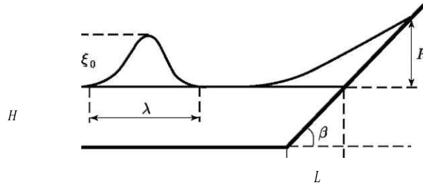
Fig. 5.12 Formulation of the problem of a tsunami run-up on the coast
