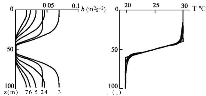
Fig. 7.6 Vertical profiles of turbulence energy and of temperature, calculated at successive time moments for L = 10\text{ m} , ft = 0.0001\text{ m}^3\text{ s}^{-3} and \tau = 100\text{ s} . Curves 1-7 correspond to t = 0, 50, 100, 150, 200, 250 and 300\text{ s}
