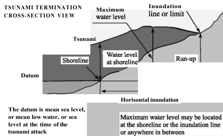
Fig. 1.3 Scheme of tsunami onshore run-up. Adapted from [UNESCO-IOC. Tsunami Glossary (2006)]
