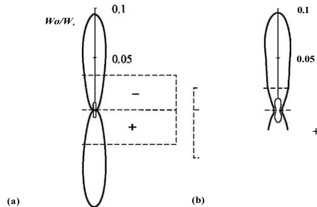
Fig. 2.39 Directional diagrams of energy emission for waves, caused by a bottom displacement alternating in sign. The shape and orientation of the source ( a_1 = a_2 = 5 (a), a_1 = 7, a_2 = 3 (b)) are shown by the dotted line. Calculations are performed for b = 10, m = 1 (thick line), m = 10 (thin line)
