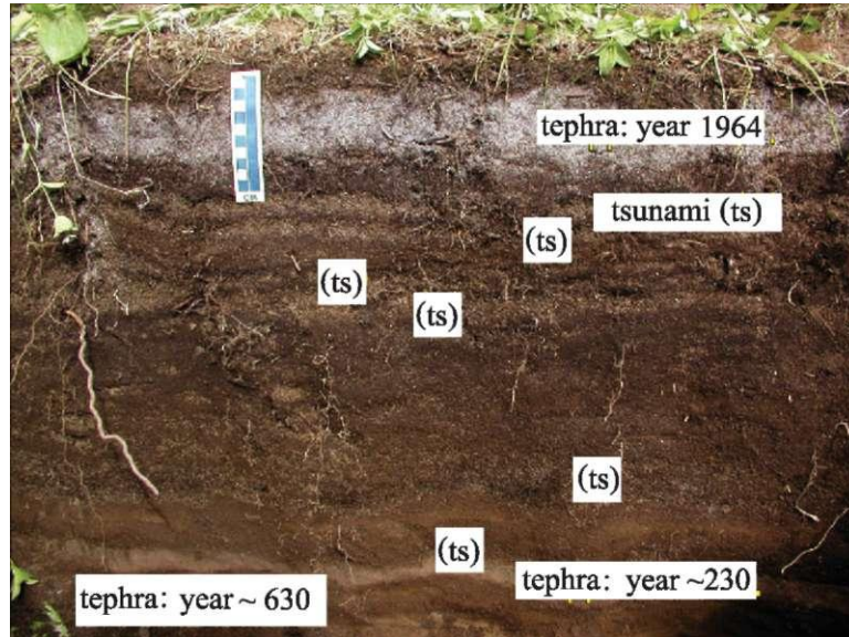
Plate 12 Photograph of wall of bore with strata of tephra and tsunamigenic horizons in the soil. The bore is located at the 20th terrace 500 m from the shore of today (peninsula of the Kamchatka cape, Kamchatka) (see also Fig. 6.10 on page 245)
