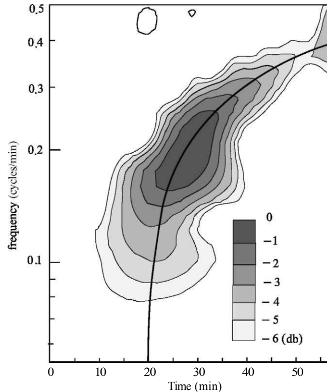
Fig. 5.2 Spectral-time diagram for amplitude of ocean-level oscillations during passage of tsunami of March 6, 1988, tsunami (the record is shown in Fig. 5.1). The isoUnes are drawn steps of 1 dB. The solid Une shows theoretical calculation of time spectral components take effect, performed in accordance with the dispersion law for gravitational waves (Adapted from [Kulikov, Gonzalez (1995)])
