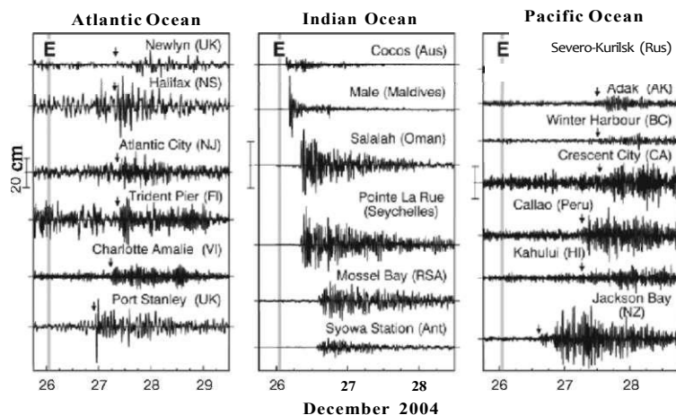
Fig. 5.9 Time series of tsunami wave heights (cm) as recorded at selected tide-gauge stations in the three major ocean basins. Arrows indicate first arrival of the tsunami (Reprinted from [Titov et al. (2005)] by permission of the publisher)
