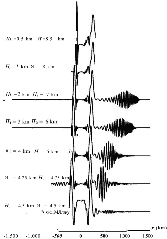
Fig. 3.10 Perturbation of free surface at time moment t = 1,000 s
