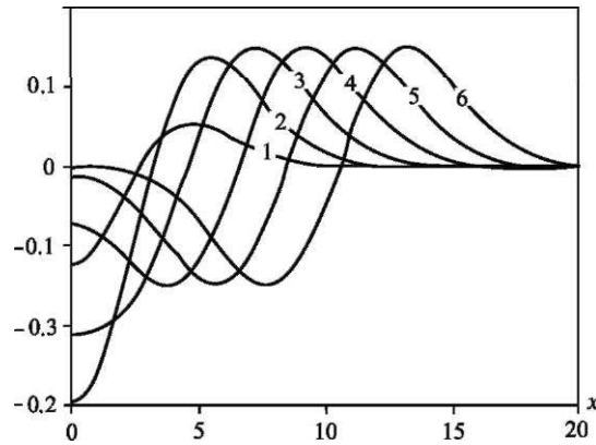
Fig. 3.21 Profile of wave formed by the non-linear mechanism in an incompressible ocean. The calculation is performed for consecutive moments of time t = 2, 4, 6, 8, 10, 12 (curves 1-6) for the case of \Gamma 1 and a = 5, m = 3
