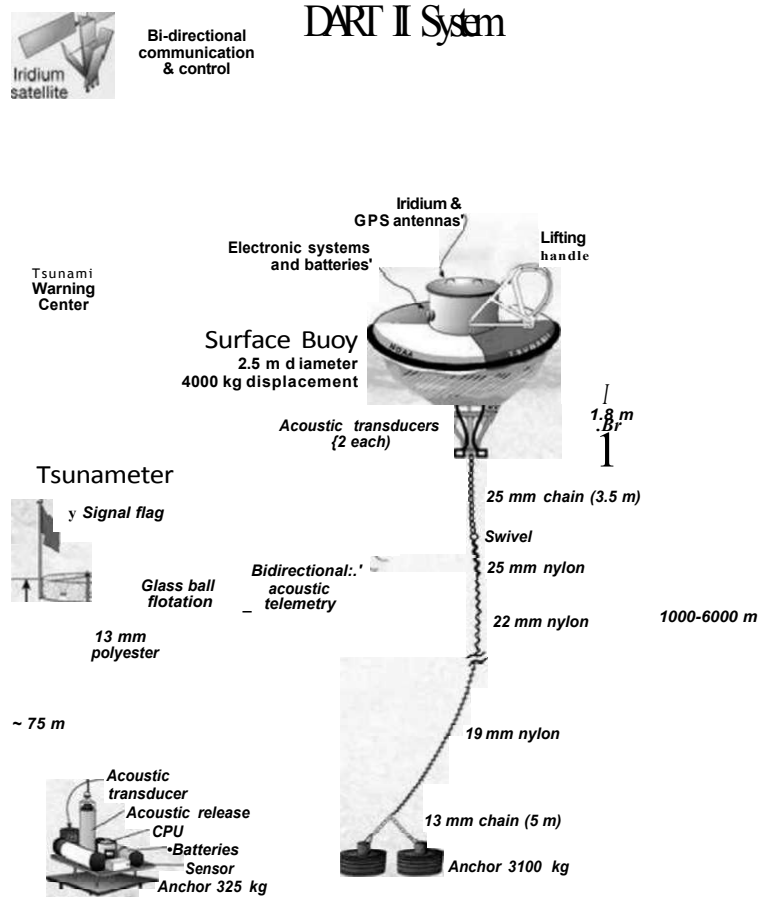
Fig. 6.5 Layout of station (DART II) for registering tsunamis in the open ocean. The figure is taken from http://www.ndbc.noaa.gov/dart.shtml (see also Plate 9 in the Colour Plate Section on page 317)
