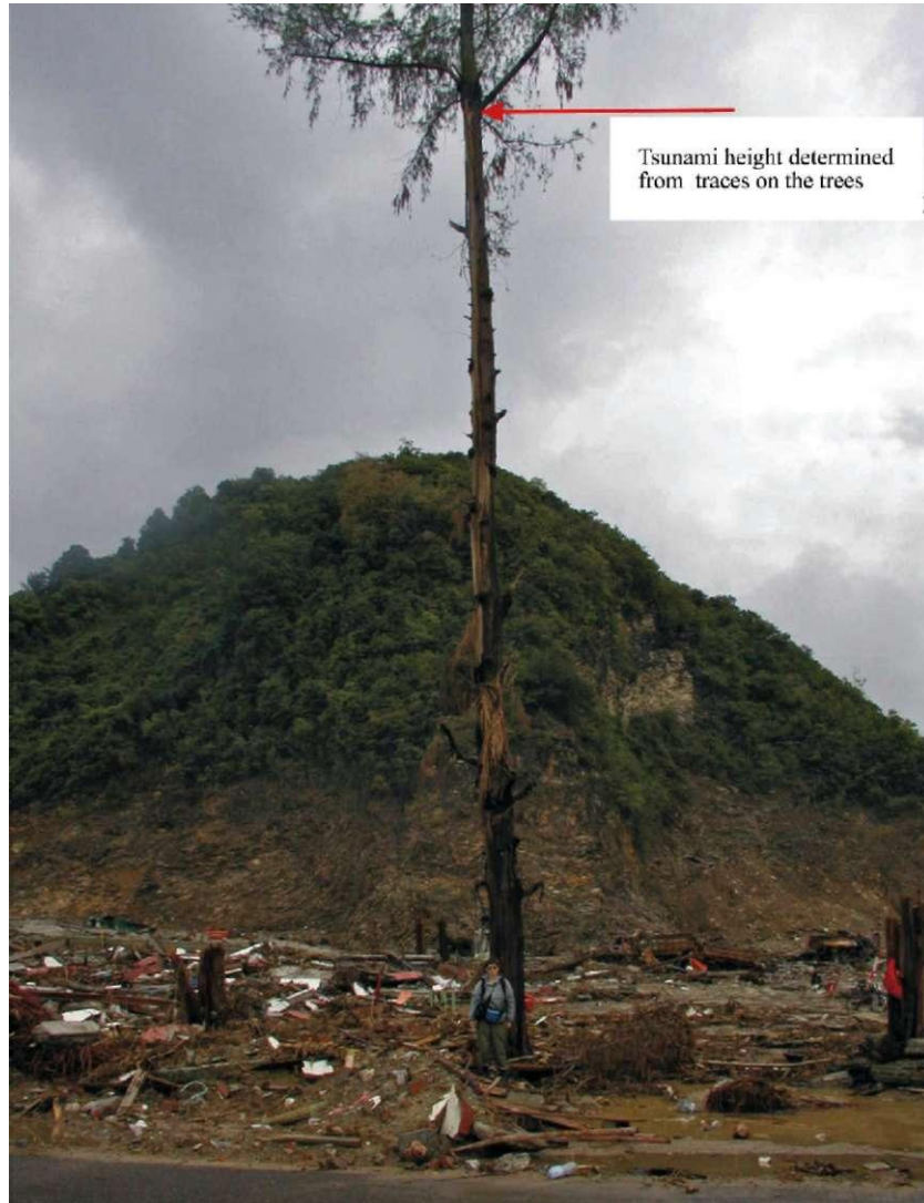
Plate 11 Segment of shore 15 km south-west of the northern end of island Sumatra. The tsunami height amounted to 15-20m, here, while the heights of individual run-ups were up to 35 m above the sea level. In this region the tsunami exerted a strong erosive and abrasive influence on the shore and the nearby hills. In the background of the photograph one can see an abrasion niche, formed after the tsunami. The distance from the shoreline is 300 m (Photo by T. K. Pinegina) (see also Fig. 6.8 on page 242)
