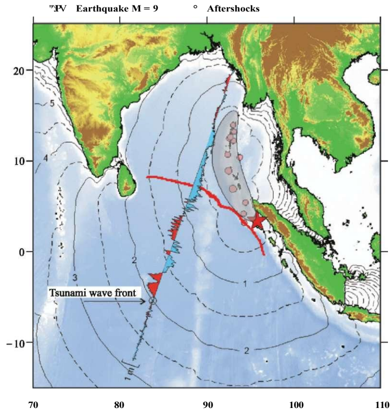
Plate 14 Map of north-eastern part of the Indian Ocean with isochrones, showing the calculated front position of the tsunami of December 24, 2004 (with an interval of 0.5 an hour). 1—epicentre of the main earthquake, 2—epicentres of main aftershocks. Route of JASON-1 satellite (circuit 109-129). The profile of the ocean level determined from altimetry data is shown along the route (Courtesy of E.A. KuUkov) (see also Fig. 6.14 on page 252)
