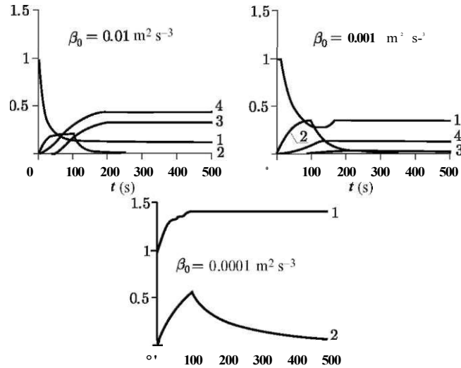
Fig. 7.7 Typical time dependences, describing variation of the maximum temperature gradient (1), of the turbulence energy averaged over depth (2), of the surface temperature (3), of the centre-of-mass position (4). Calculations are performed for L = 10\text{m} , t = 100\text{s} and different \beta_0 values (shown in the figure)
