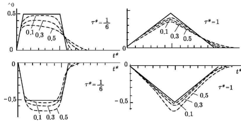
Fig. 2.20 Waves formed by a piston-like displacement of large amplitude. Calculations are performed within the framework of long-wave theory: solid line—linear theory, dotted line—nonlinear theory. The numbers, indicating the curves, show the ratio of the basin bottom deformation amplitude and the basin depth
