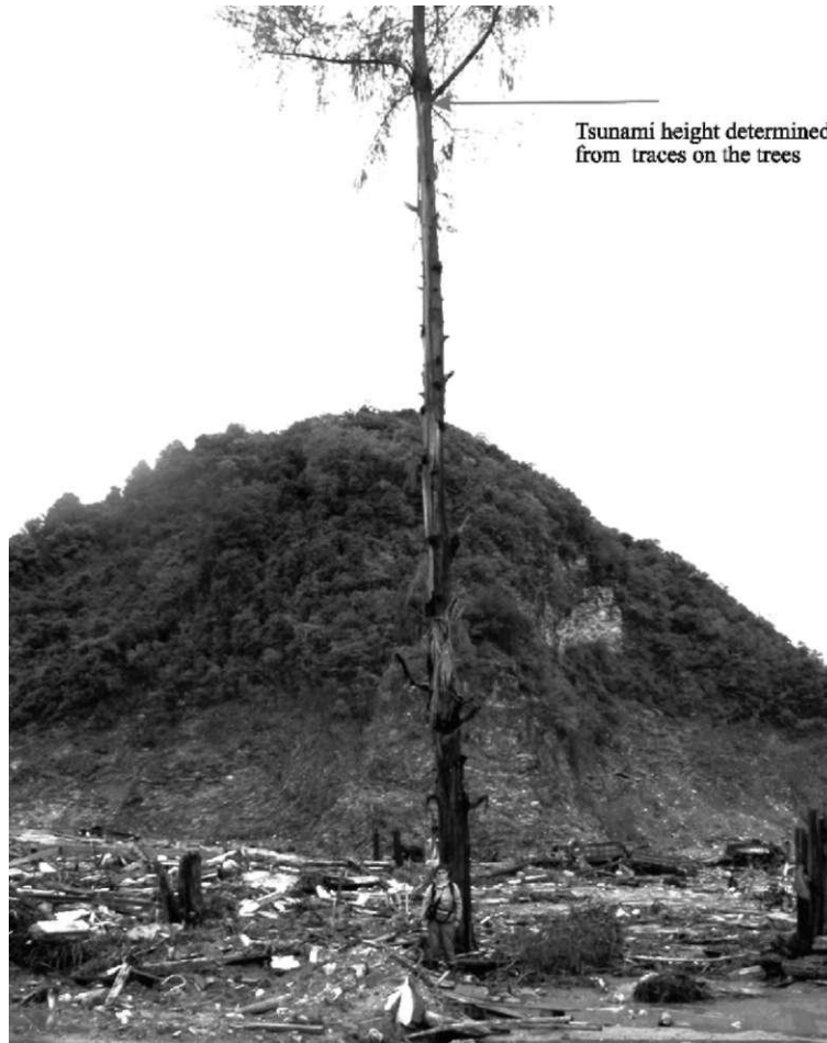
Fig. 6.8 Segment of shore 15 km south-west of the northern end of island Sumatra. The tsunami height amounted to 15-20m, here, while the heights of individual run-ups were up to 35 m above the sea level. In this region the tsunami exerted a strong erosive and abrasive influence on the shore and the nearby hills. In the background of the photograph one can see an abrasion niche, formed after the tsunami. The distance from the shoreline is 300 m (Photo by T. K. Pinegina) (see also Plate 11 in the Colour Plate Section on page 319)
