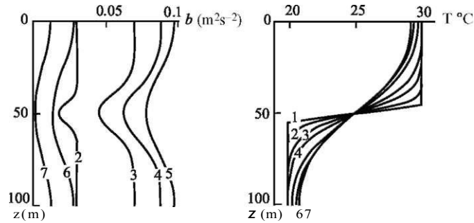
Fig. 7.5 Vertical profiles of temperature and of turbulence energy, calculated at successive moments of time for L = 10\text{m} , ft = 0.003\text{ m}^3\text{ s}^{-3} and \tau = 100\text{ s} . Curves 1-7 correspond to t = 0, 10, 30, 50, 100, 150 and 200\text{ s}
