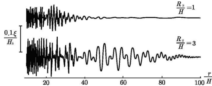
Fig. 4.9 Profile of waves excited by underwater eruption. The calculation is performed for t = 100\pi/H/g for two different ratios of the initial perturbation radius and the ocean depth, R_s/H (the values are indicated in the figure)
