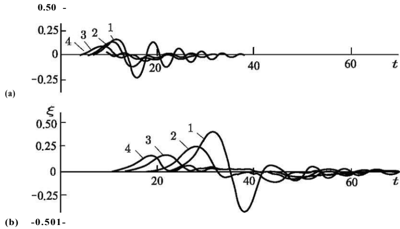
Fig. 2.30 Time-base of waves caused by piston-like displacement. Calculations are performed at points lying on a circle of radius r = 10 (a) and r = 30 (b) with its centre at the origin of the reference frame, for azimuthal angles a = 0, 30, 60, 90^\circ (curves 1–4, respectively). The parameters of the bottom displacement: a = 1, b = 5, m = 1 (a) and a = 3, b = 15, \tau = 1 (b)
