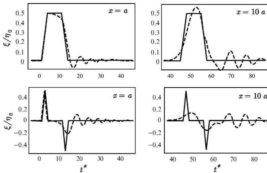
Fig. 2.11 Waves formed by piston (upper row) and membrane (lower row) displacements of duration m^* = 3 close to the right boundary of the generation area ( x = a ) and at a significant distance from it ( x = 10a ). The horizontal extension of the source 2a = 10 . The solid line represents the linear theory of long waves, the dotted one the linear potential theory
