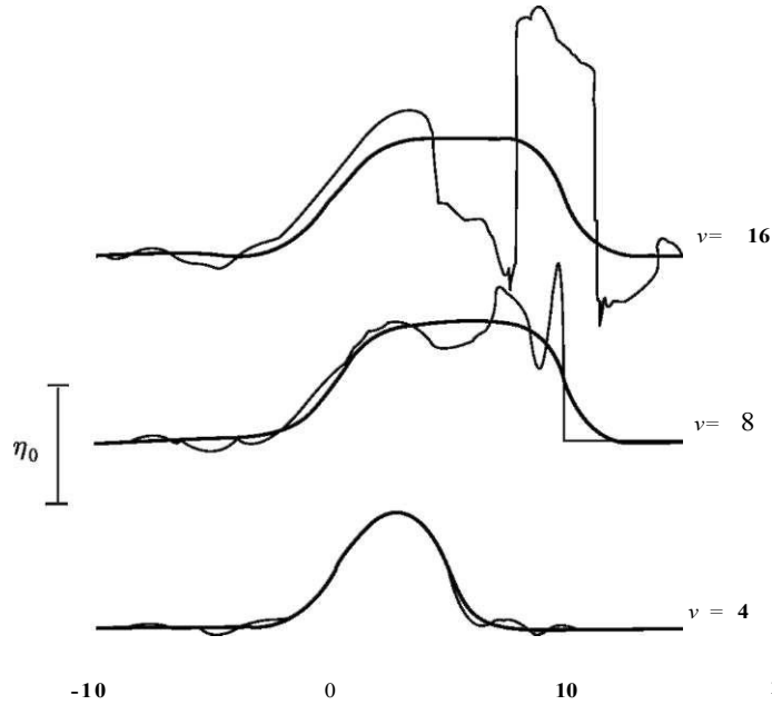
Fig. 3.5 Profiles of surface displacement of a liquid at moment of time t = 10 for different propagation velocities of the running displacement, v . The thick and thin lines correspond to incompressible and compressible liquids, respectively
