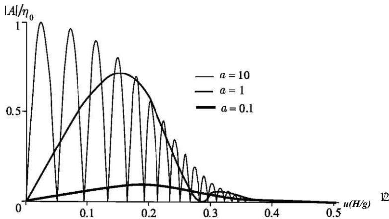
Fig. 2.27 Amplitude of progressive wave excited by oscillating area of ocean bottom versus the frequency of bottom oscillations for different sizes of the source, a
