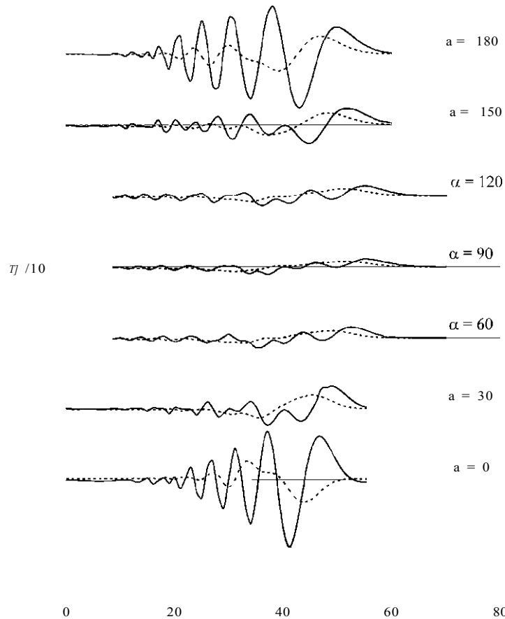
Fig. 2.38 Wave profiles (perturbation of free surface as function of radius r ) for various azimuthal angles \alpha at time moment t = 50 . The parameters of the displacement are a| = 7 , ai = 3 , b = 10 , \tau = 1 (solid line), \tau = 10 (dotted line)
